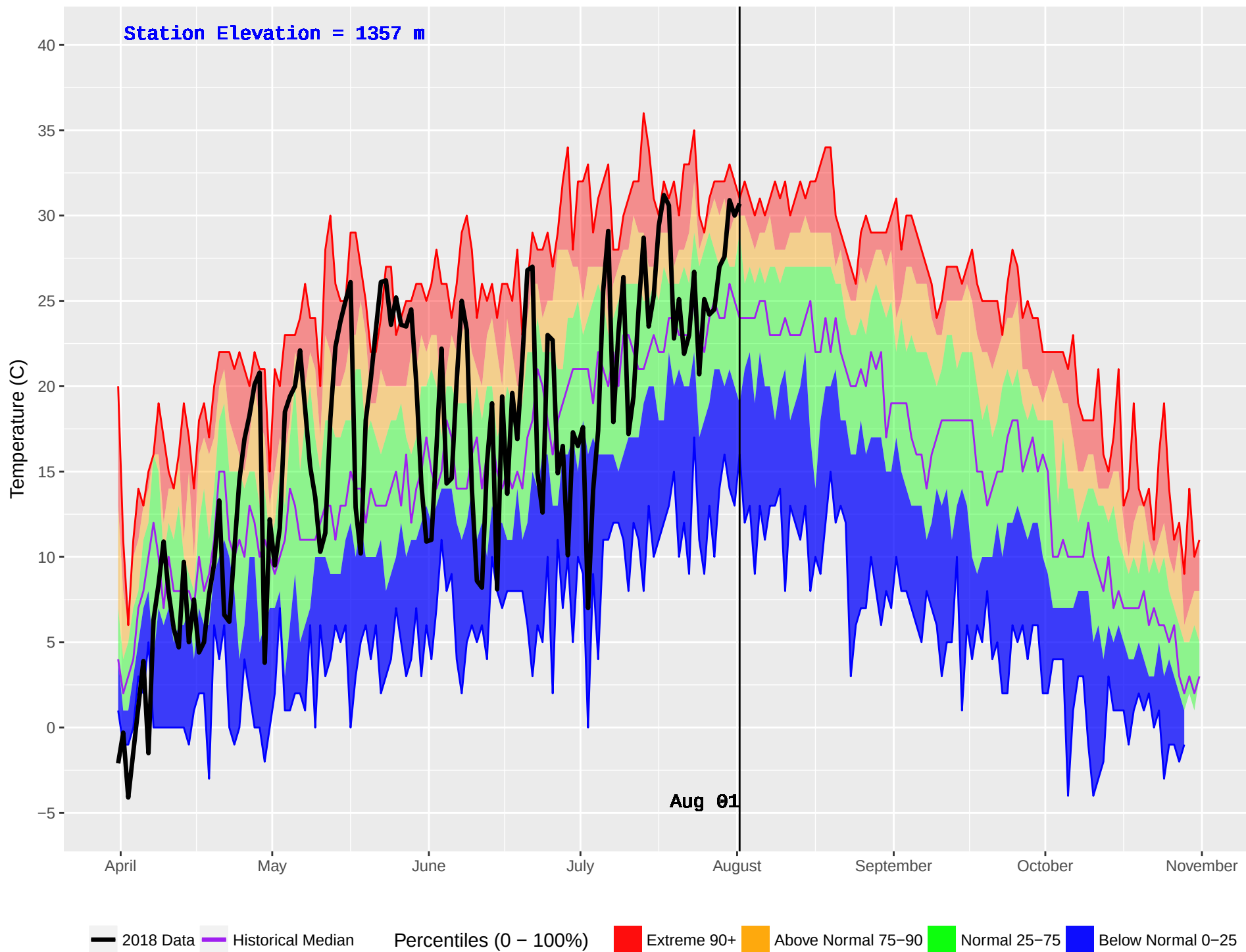
WHITE RIVER (790) : Historical (1989–2016) and Current (2018) Daily Temperature
