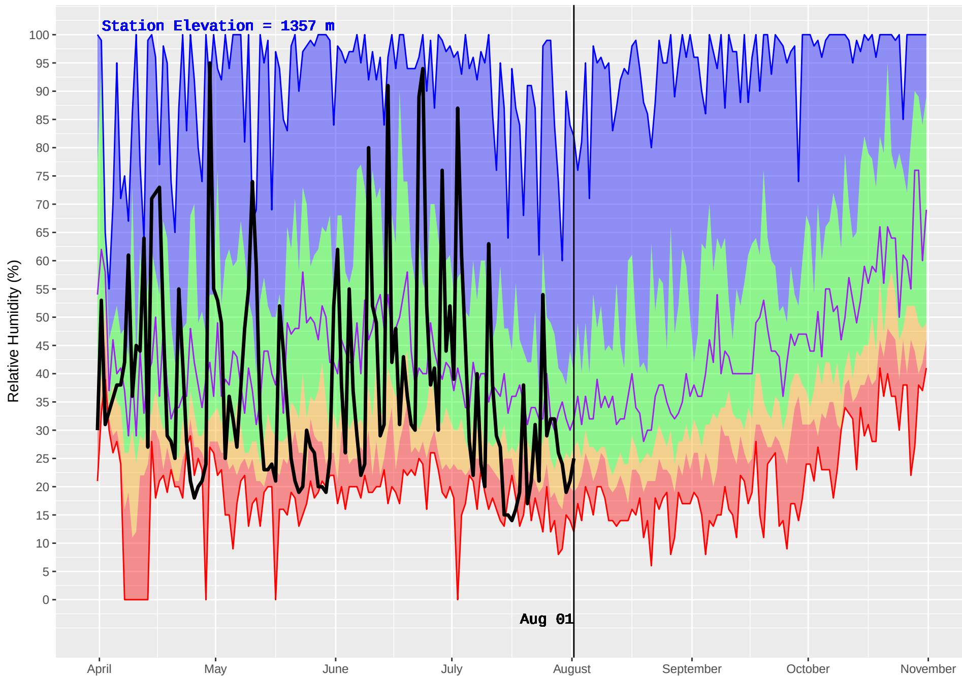
WHITE RIVER (790) : Historical (1989–2016) and Current (2018) Daily Relative Humidity
