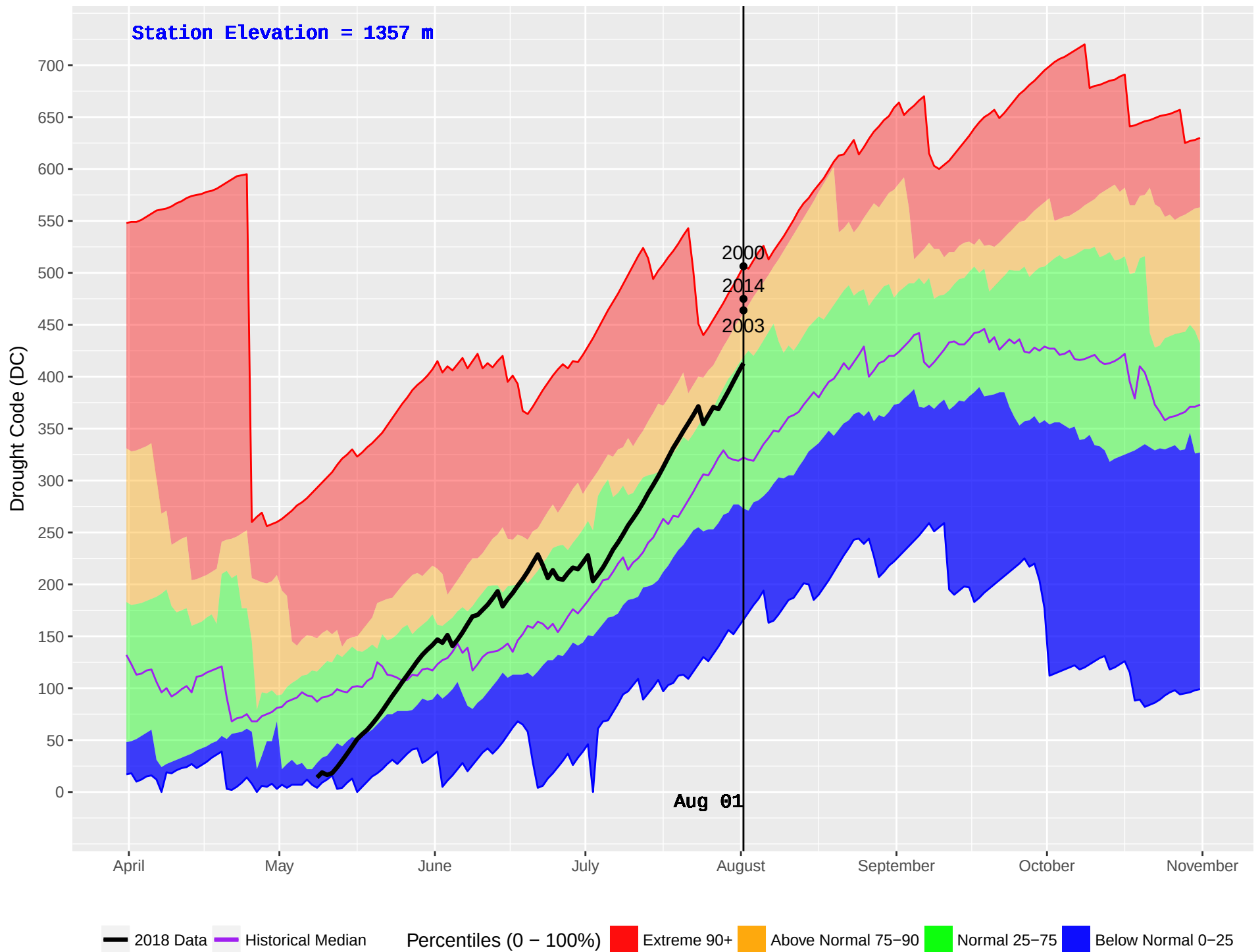
WHITE RIVER (790) : Historical (1989–2016) and Current (2018) Daily Drought Code (DC)
