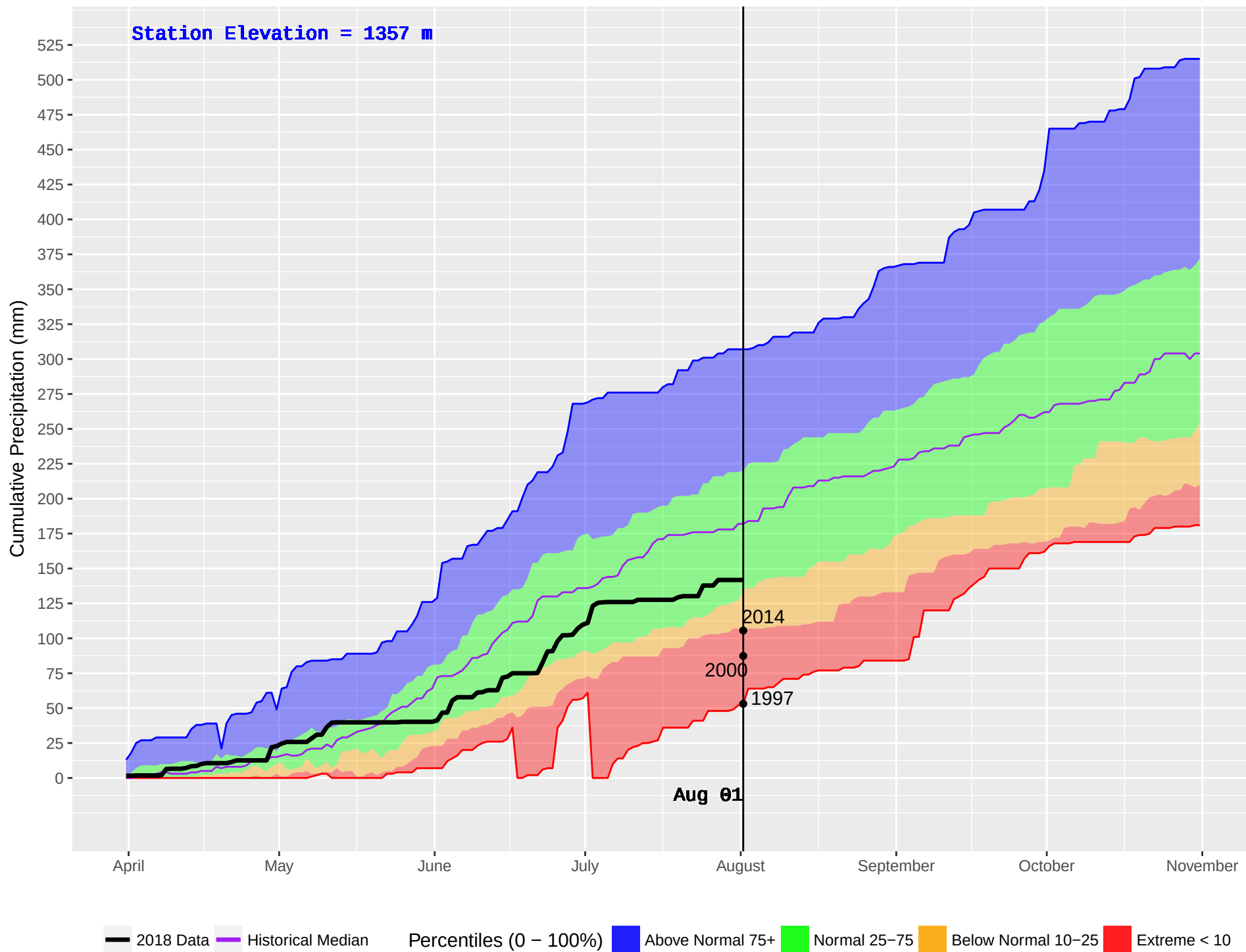
WHITE RIVER (790) : Historical (1989–2016) and Current (2018) Daily Cumulative Precipitation
