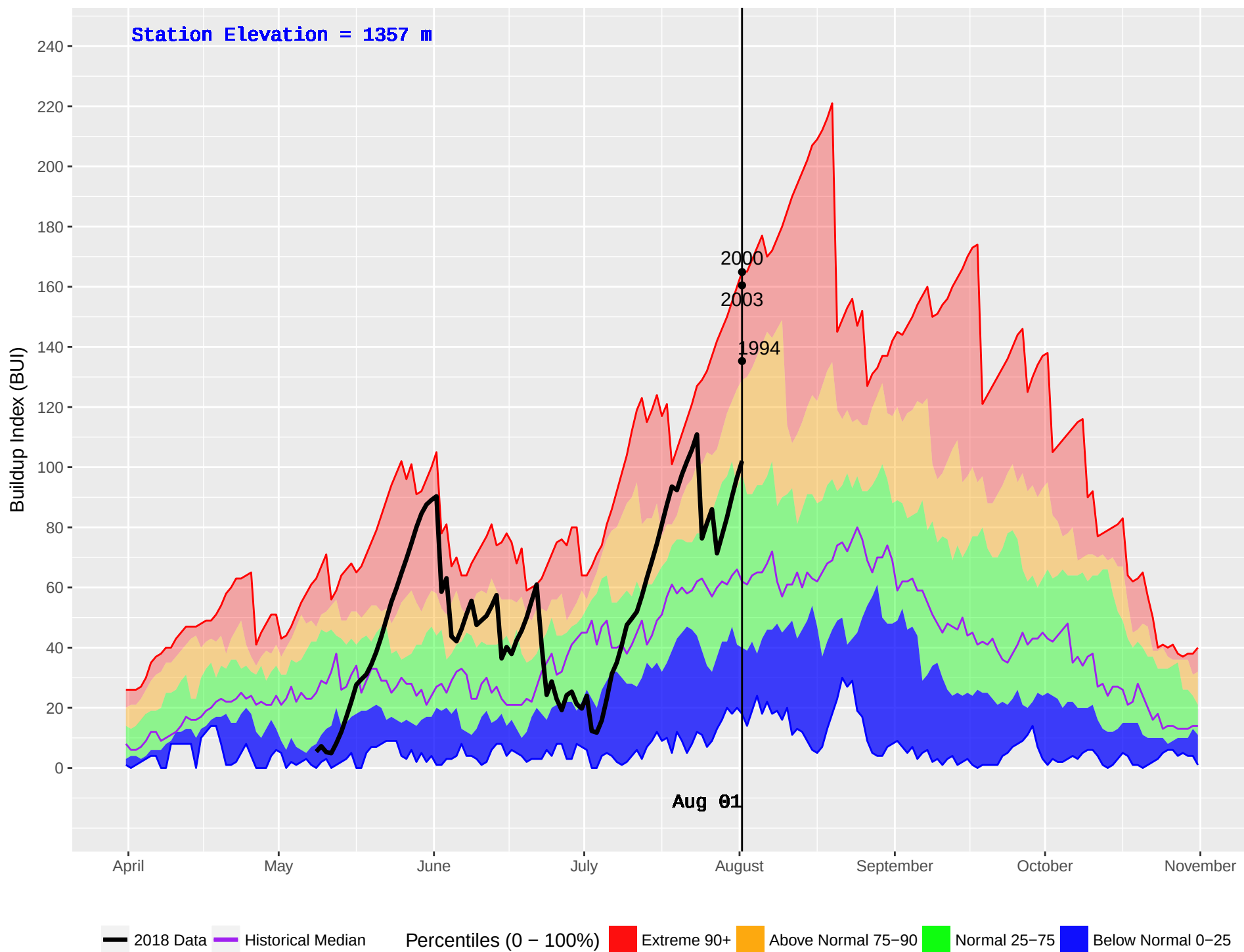
WHITE RIVER (790) : Historical (1989–2016) and Current (2018) Daily Buildup Index (BUI)
